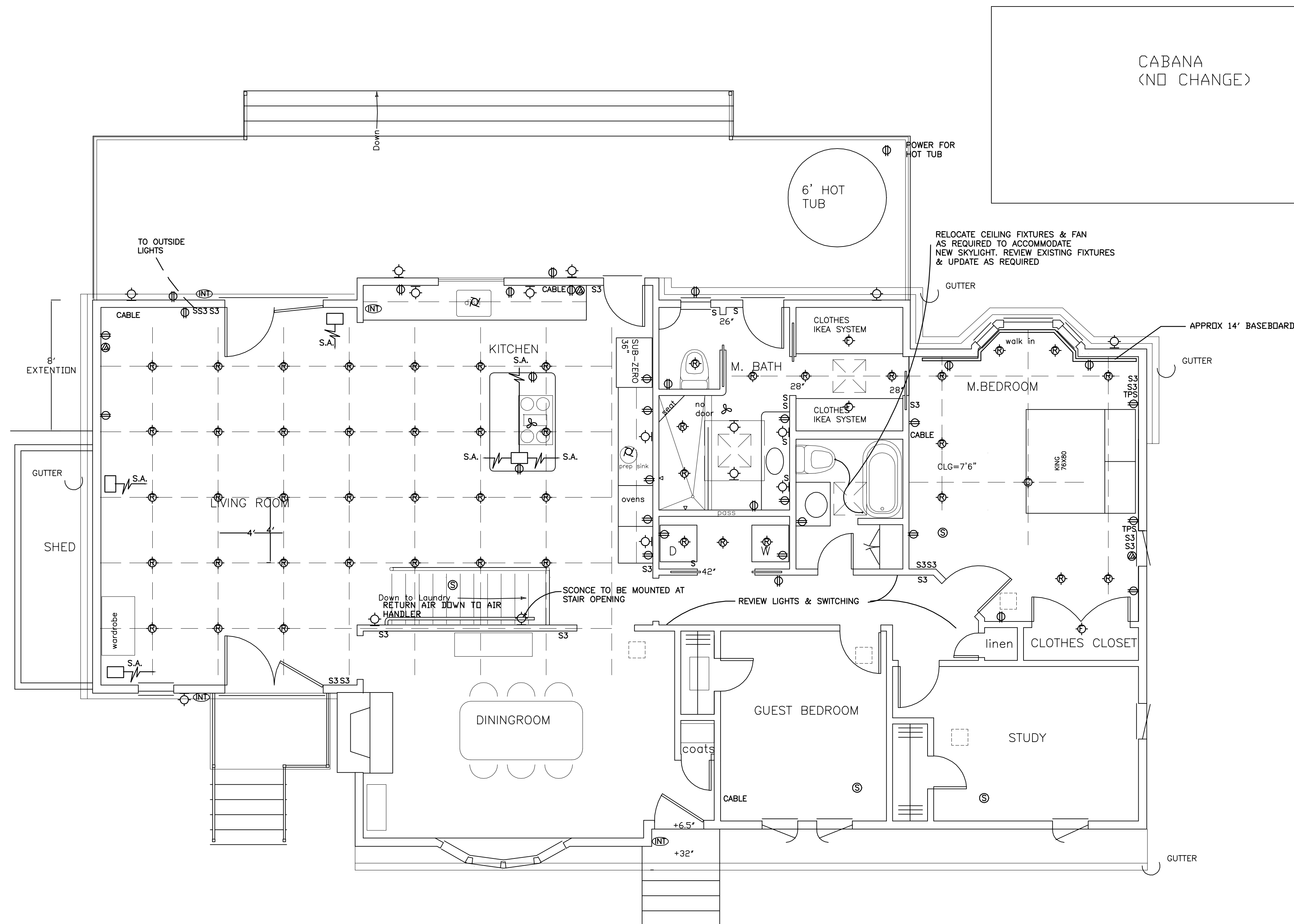
PROPOSED /MECHANICAL FIRST FLOOR PLAN
