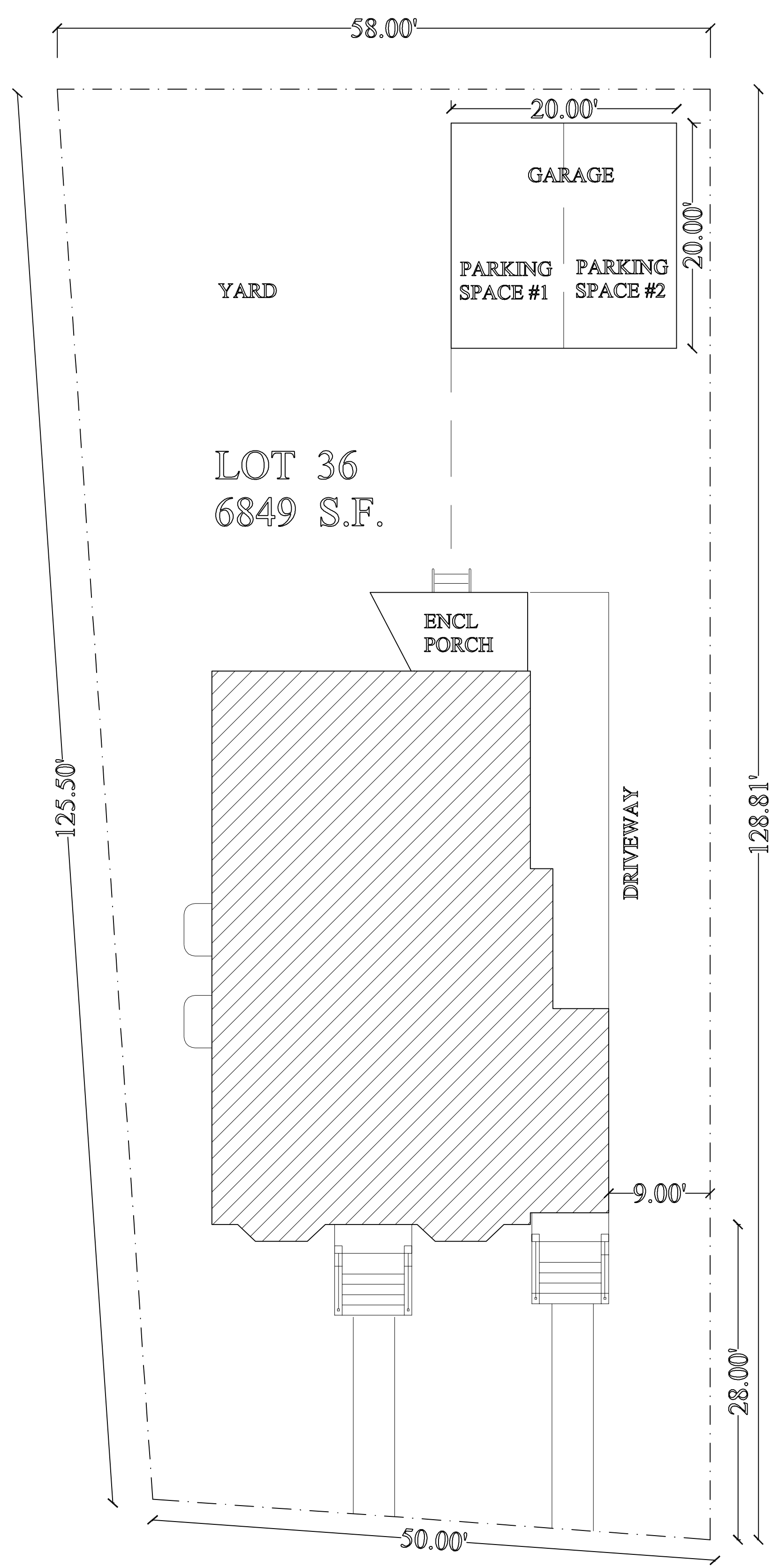
SITE PLAN
