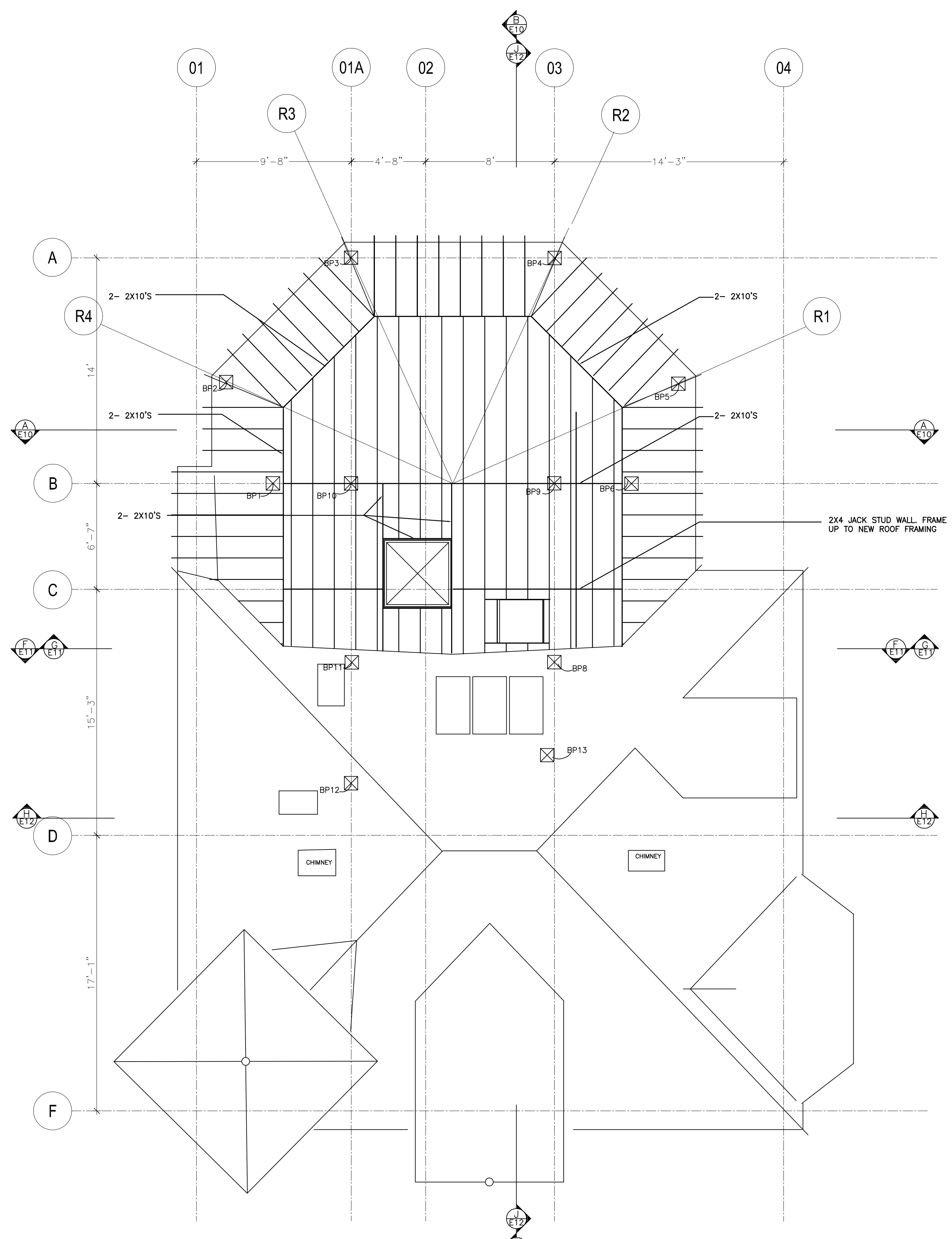
FRAMING PLAN ROOF PLAN SCALE 1/4" = 1'-0"
