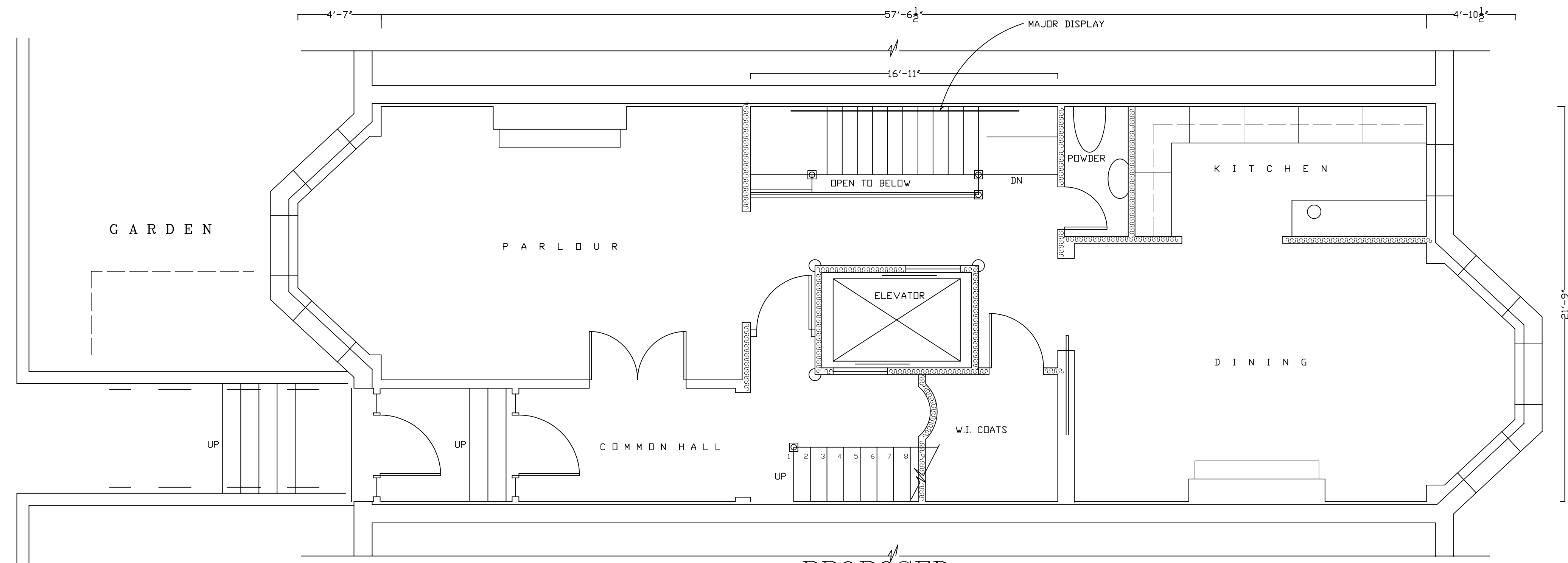
PROPOSED FIRST FLOOR
