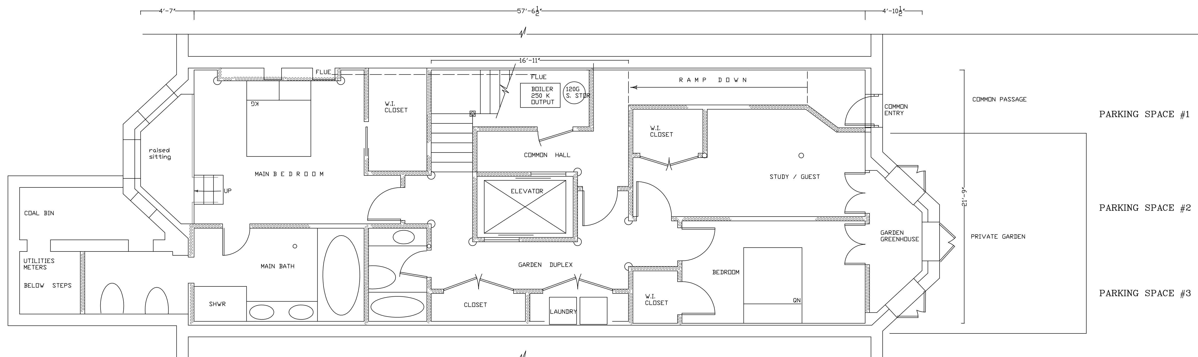
PROPOSED GARDEN FLOOR
