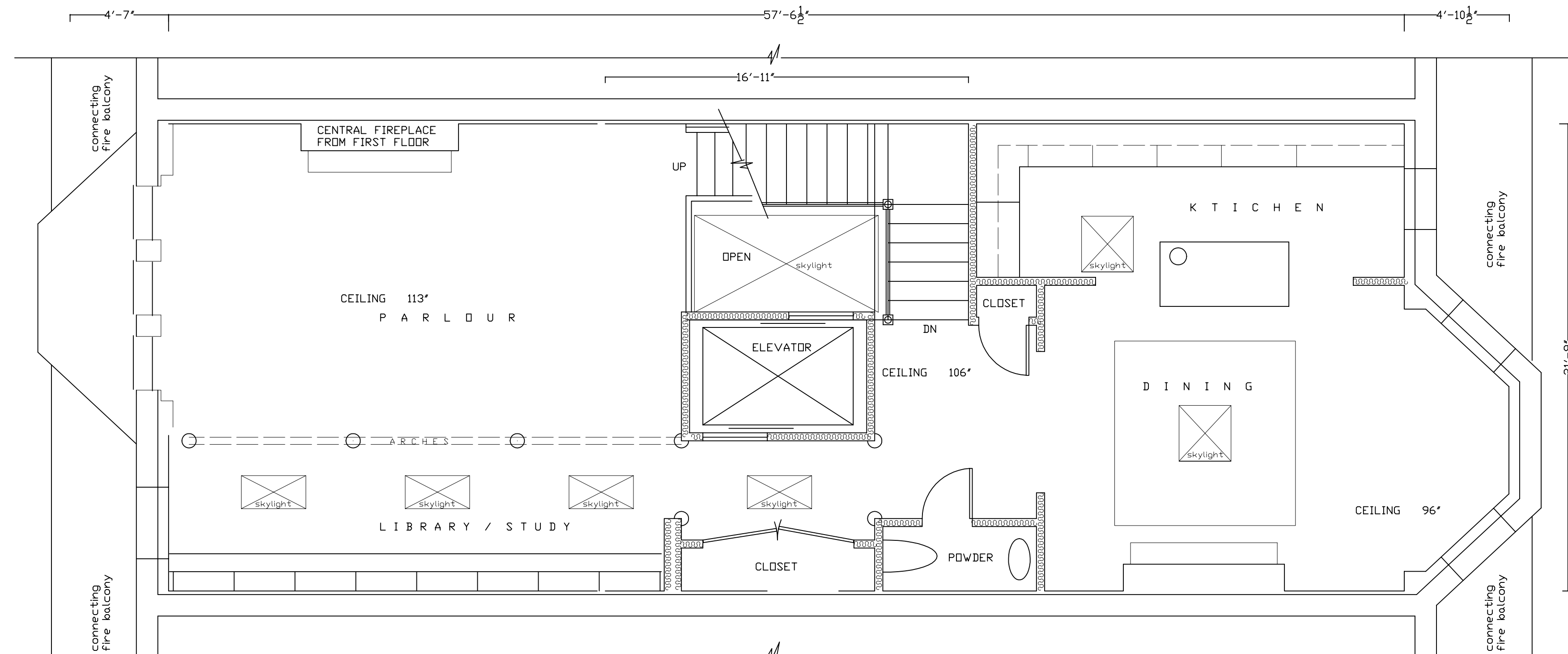
PROPOSED FOURTH FLOOR
