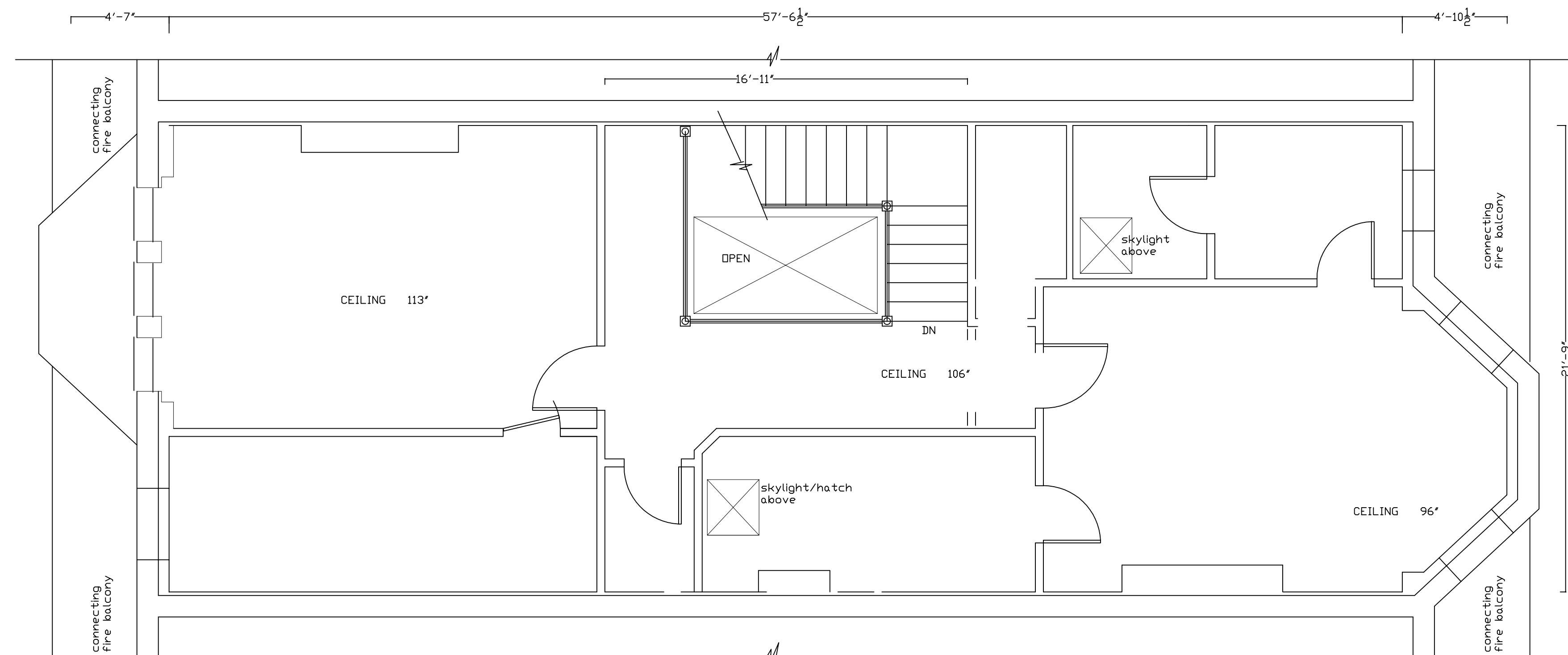
EXISTING FOURTH FLOOR
