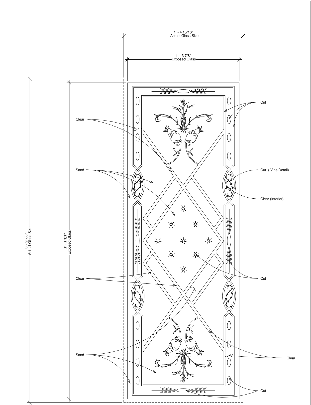
① Front Door Glass Detail 3" = 1'-0"
